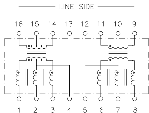
Circuit B
