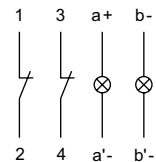
Wiring diagram 12
