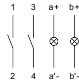
Wiring diagram 10
