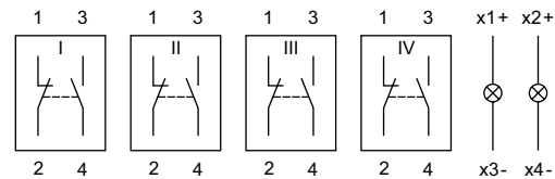
Wiring diagram 7
