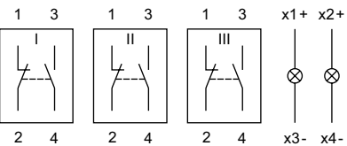
Wiring diagram 6
