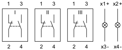
Wiring diagram 5
