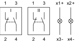
Wiring diagram 4
