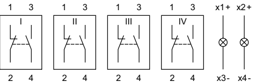
Wiring diagram 8
