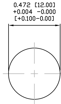
PANEL CUTOUT
