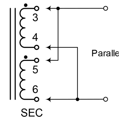
Secondary Wiring (Parallel Connection)
