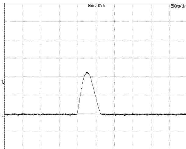
Figure 11: Inrush current @ Vin=72V CH1:Iin, 2A/div, 200nS/div; Max current 4.3A, I2t=1.5E-7 A²S
