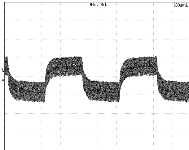
Figure 7: Dynamic response to load step 6.25A~9.375A with 0.1A/uS slew rate at 72Vin CH1:VOUT, 100mV/div, 500uS/div
