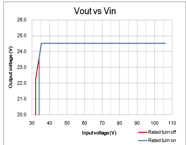
Figure 2: V_{out} vs. V_{in} @ Full load
