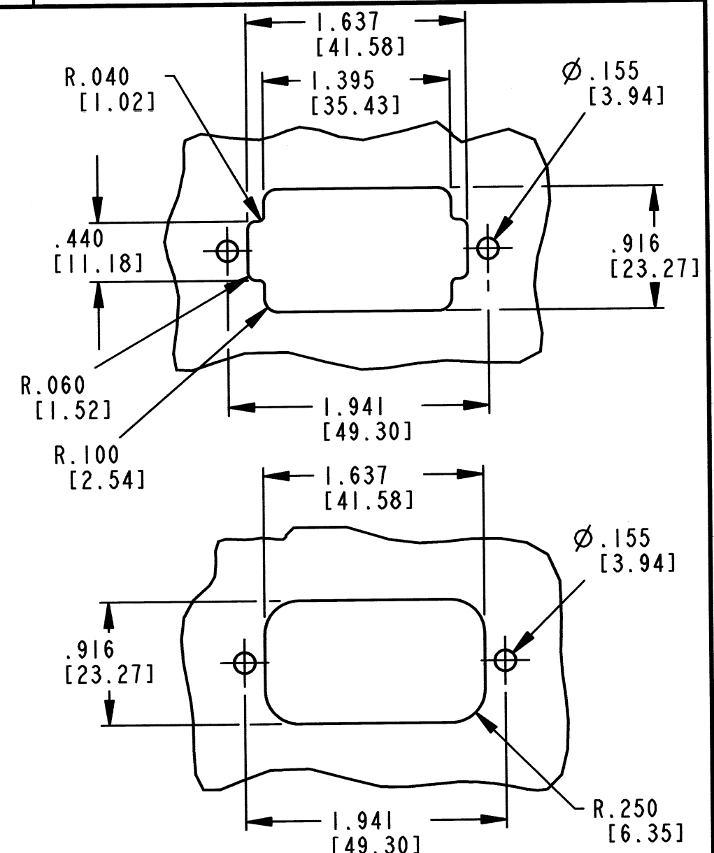
RECOMMENDED PANEL CUTOUTS
