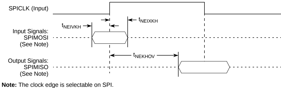
Figure 55. SPI AC Timing in Slave Mode (External Clock) Diagram
