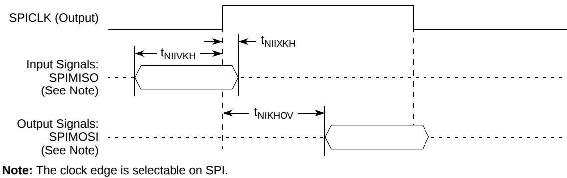
Figure 56. SPI AC Timing in Master Mode (Internal Clock) Diagram
