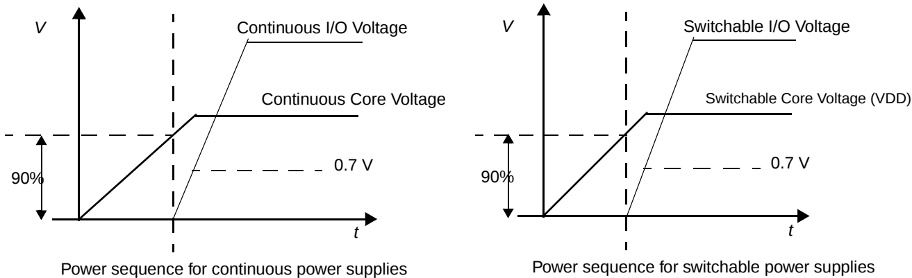
Figure 3. Power-Up Sequencing
