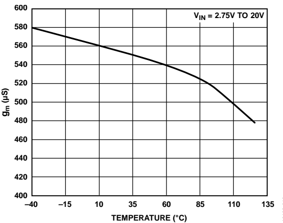
Figure 18. g_m of Error Amplifier vs. Temperature
