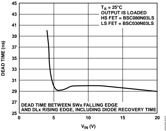
Figure 17. Dead Time vs. V_{IN}
