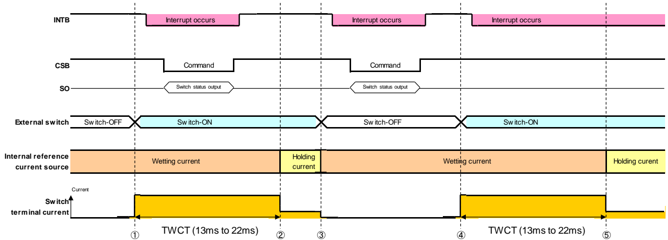
Figure 17. Wetting Current Timer (Continuous Operation)
