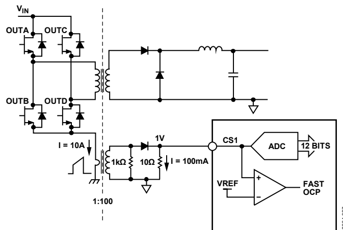
Figure 29. Current Sense 1 (CS1) Operation
