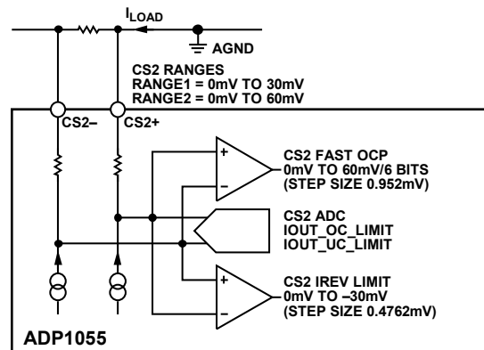
Figure 30. Differential Low-Side Sensing
