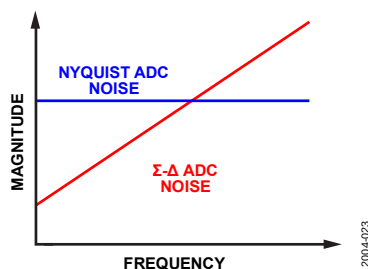
Figure 28. Noise Performance for Nyquist Rate and \Sigma\text{-}\Delta ADCs
