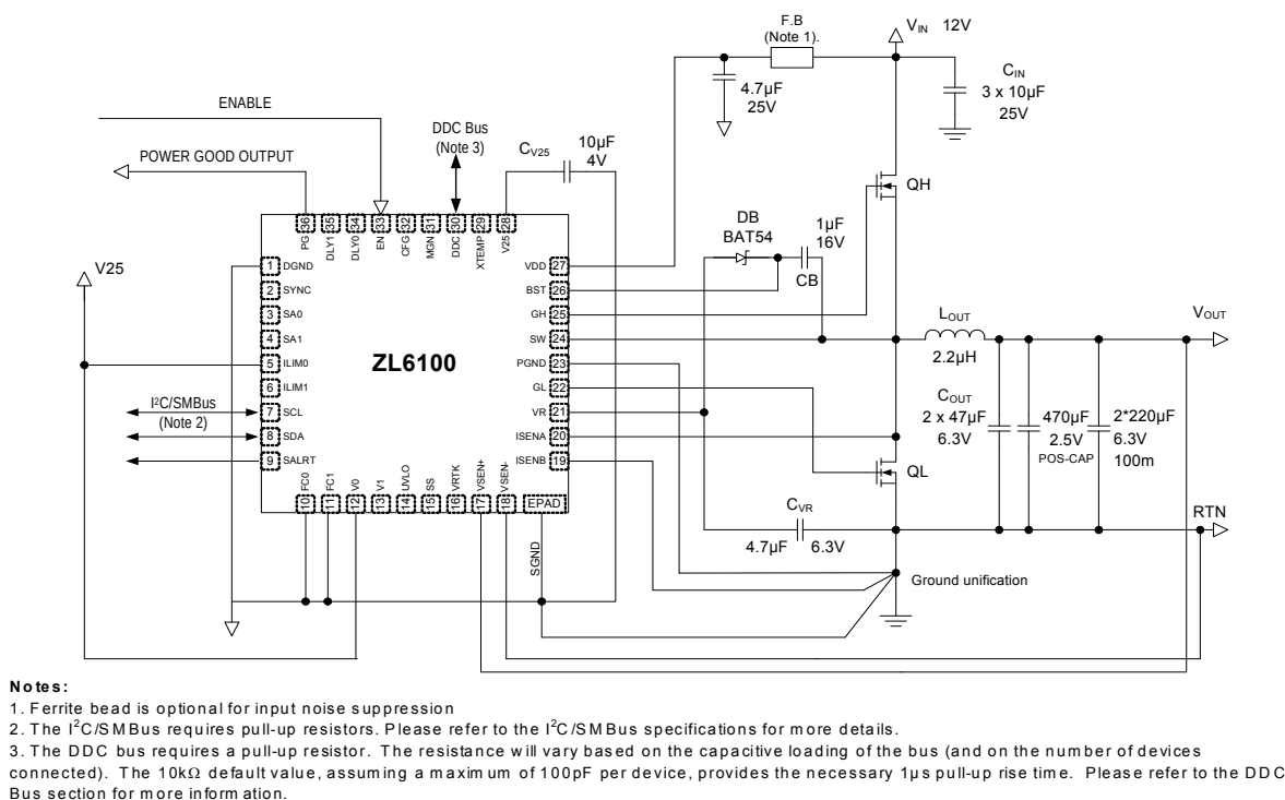
FIGURE 2. 12V TO 1.8V/20A APPLICATION CIRCUIT (4.5V UVLO, 10ms SS DELAY, 5ms SS RAMP)
