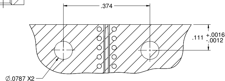
PCB LAYOUT
