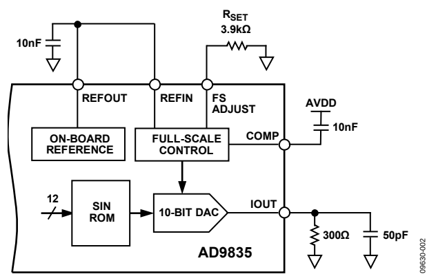
Figure 2. Test Circuit
