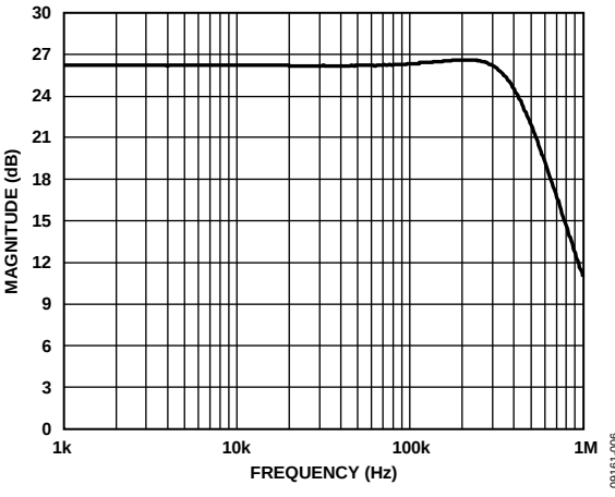
Figure 6. Typical Small-Signal Bandwidth ( V_{OUT} = 200\text{ mV p-p} )
