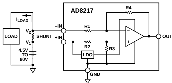
Figure 24. Simplified Schematic
