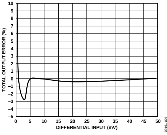
Figure 7. Total Output Error vs. Differential Input Voltage
