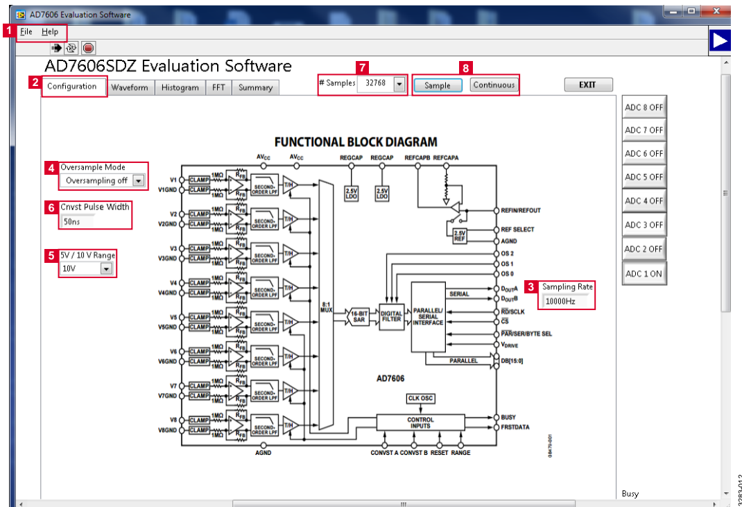
Figure 11. AD7606 Evaluation Software Main Window
