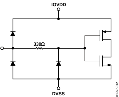
Figure 10. Digital Inputs
