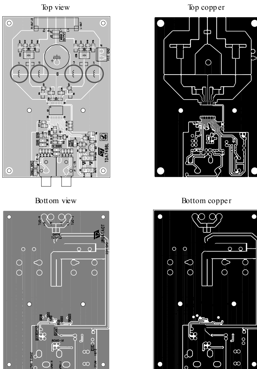
Figure 3. Test board
