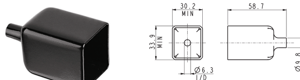
Insulation Boot
