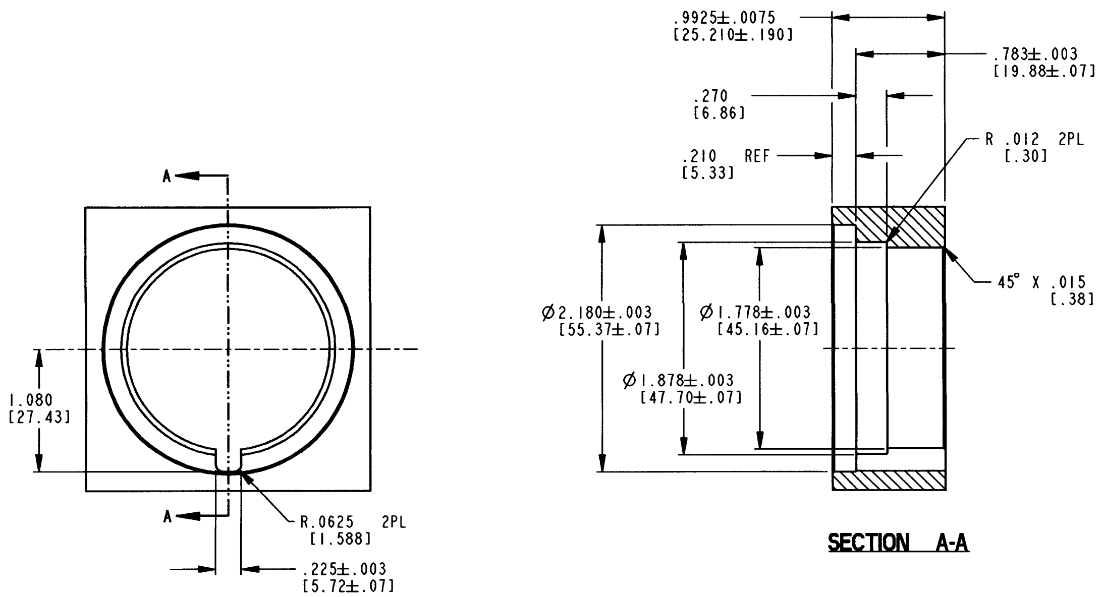
MOUNTING DETAIL FOR RECEPTACLE ALL DIMENSIONS ARE ±.005 UNLESS OTHERWISE SPECIFIED
