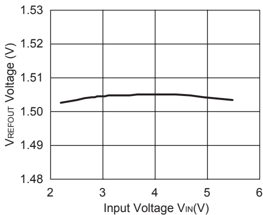
23) V_{\text{REFOUT}} Voltage vs. Input Voltage (T opt =25°C) 24) V_{\text{REFOUT}} Voltage vs. Output Current (1) (T opt =25°C) R1212D10xx
