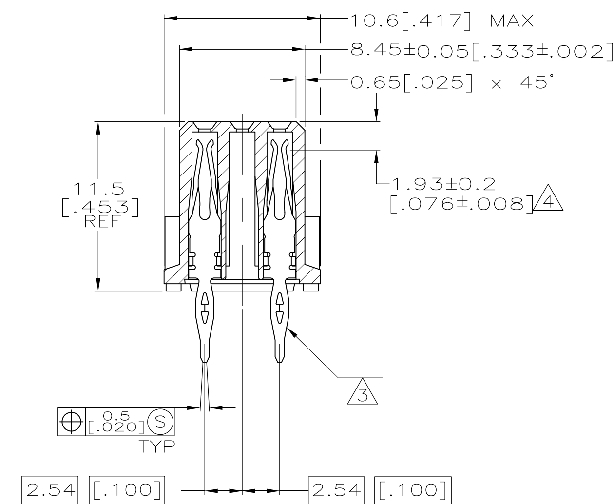
SECTION X-X
