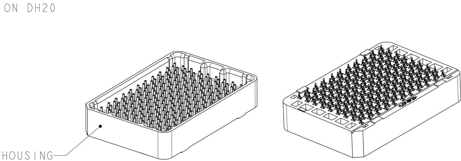
ISOMETRIC VIEW TYPICAL CONFIGURATION FOR 8mm THRU 13mm 8mm SHOWN SCALE 2:1
