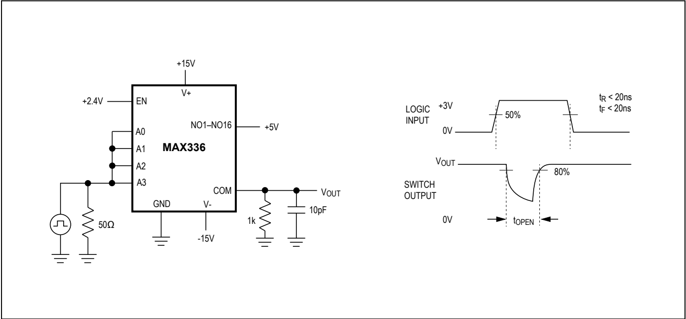
Figure 4. Break-Before-Make Interval
