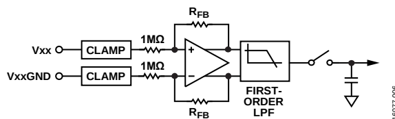
Figure 42. Analog Input Circuitry
