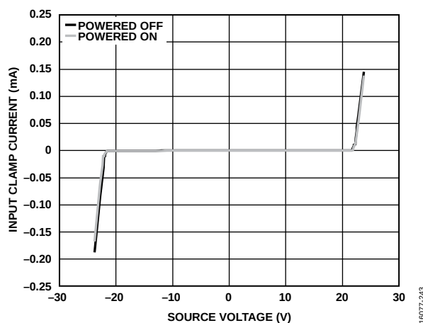
Figure 43. Input Protection Clamp Profile, Input Clamp Current vs. Source Voltage
