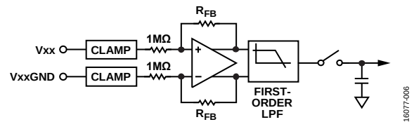
Figure 42. Analog Input Circuitry
