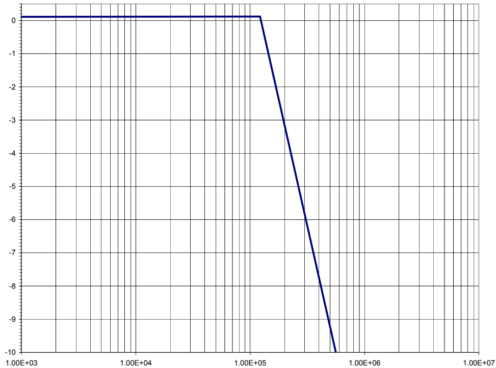
Figure 19: Jitter Transfer
