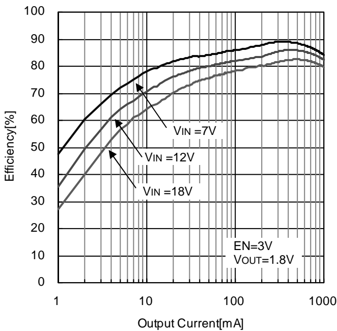
Figure 20. Efficiency - Output Current (VOUT = 1.8V)
