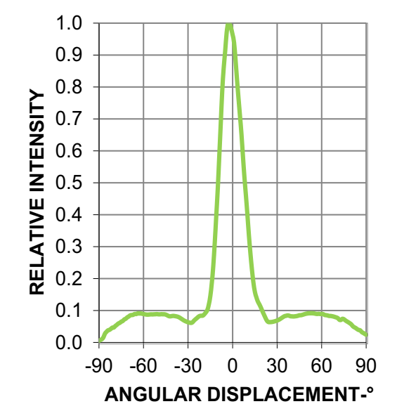
Figure 5: Radiation Pattern
