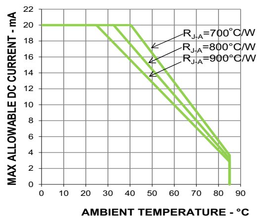
Figure 10: Derating Curve
