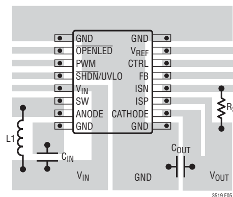
Figure 5. Suggested Layout
