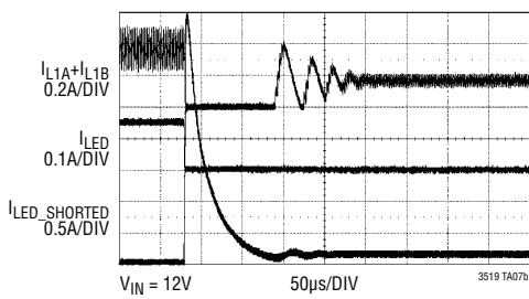
Waveforms for LED Shorted to Ground
