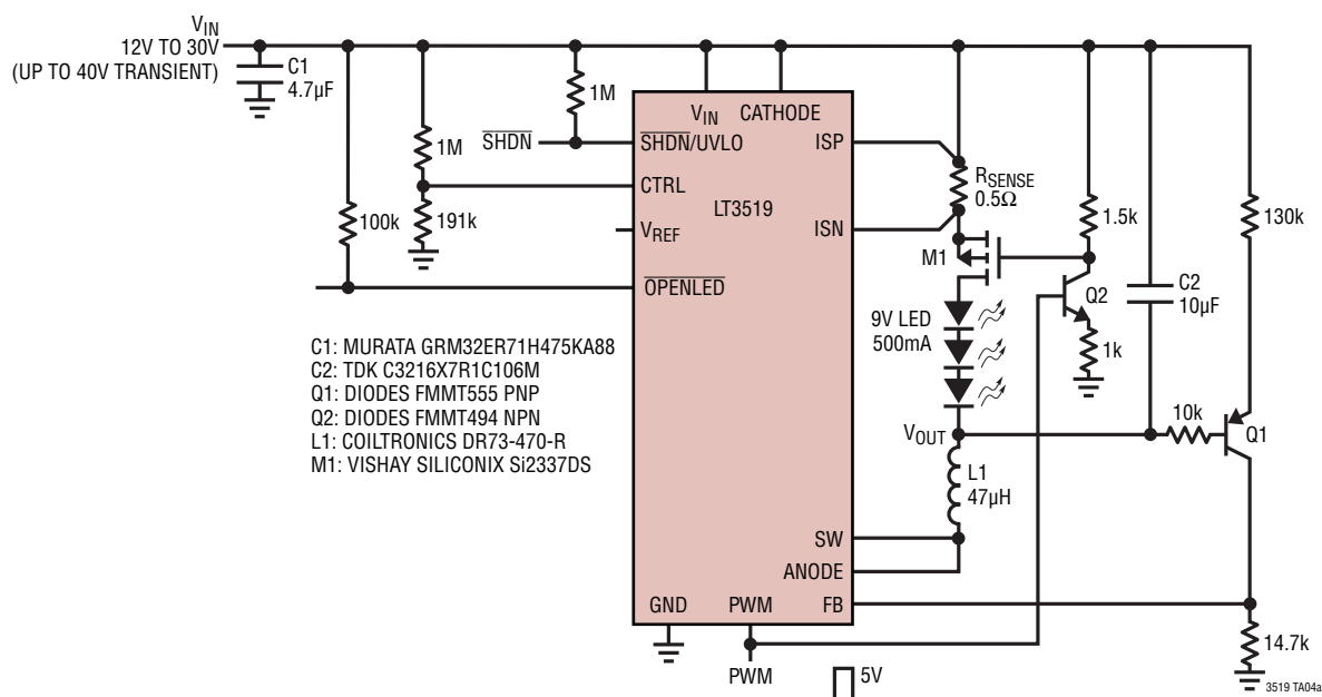
Buck Mode 500mA LED Driver
