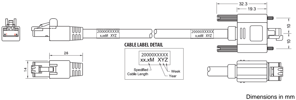
Fig. 1: Cable Overview
