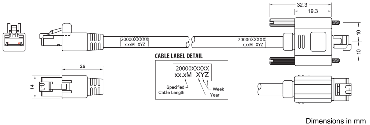
Fig. 1: Cable Overview
