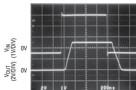
Output-Overdrive Recovery
