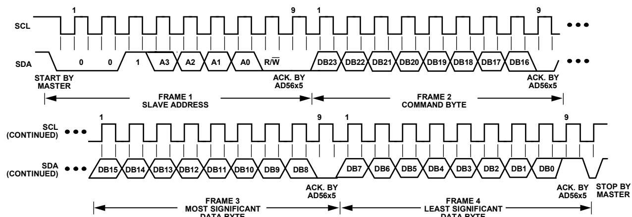
Figure 60. I²C Write Operation (14-Lead Package)
