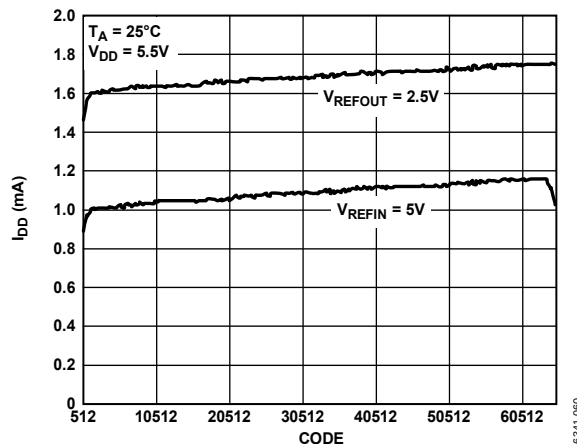
Figure 36. Supply Current vs. DAC Code
