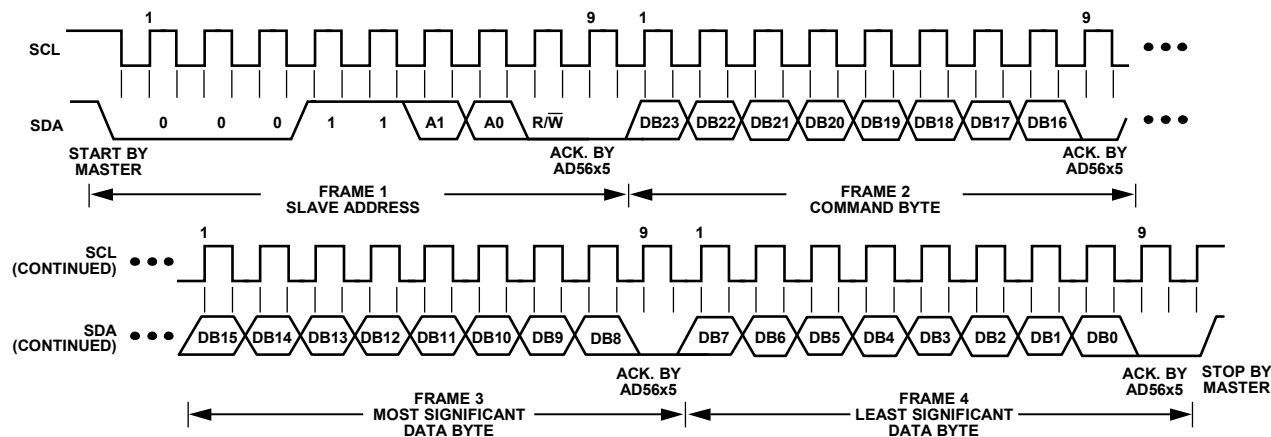
Figure 59. I²C Write Operation (10-Lead and 12-Ball Packages)
