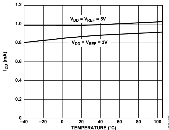
Figure 38. Supply Current vs. Temperature
