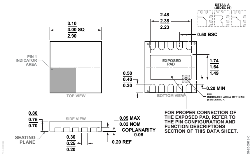
Figure 76. 10-Lead Lead Frame Chip Scale Package [LFCSP] 3 mm x 3 mm Body and 0.75 mm Package Height (CP-10-9)
