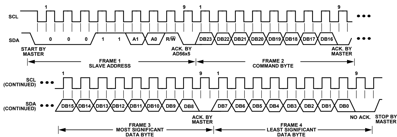
Figure 61. I²C Read Operation (10-Lead and 12-Ball Packages)
