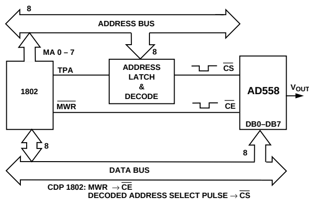
c. 1802/AD558 Interface Figure 12. Interfacing the AD558 to Microprocessors
