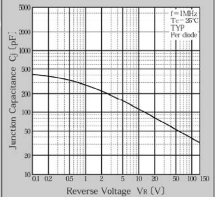
Junction Capacitance
