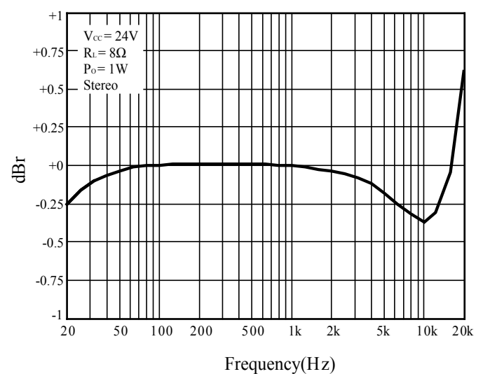
Figure 27 Frequency Response
