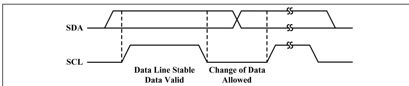
Figure 33 Bit Transfer
