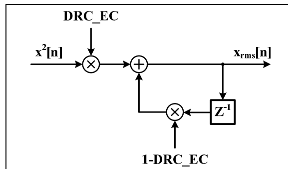
Figure 38 Digital Processing Of Calculating RMS Signal Power
