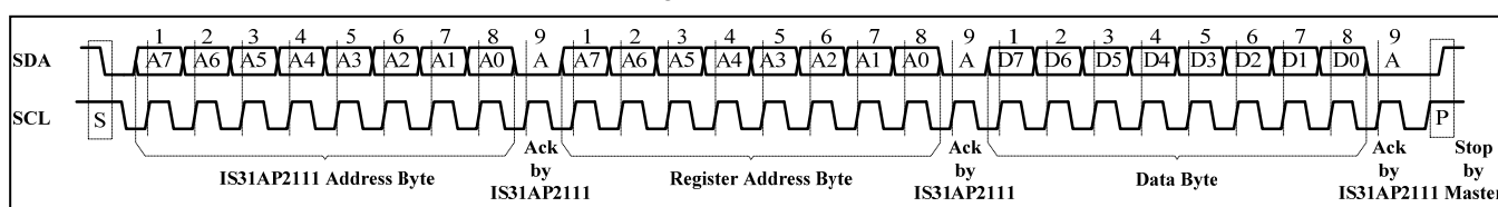
Figure 34 Writing to IS31AP2111
