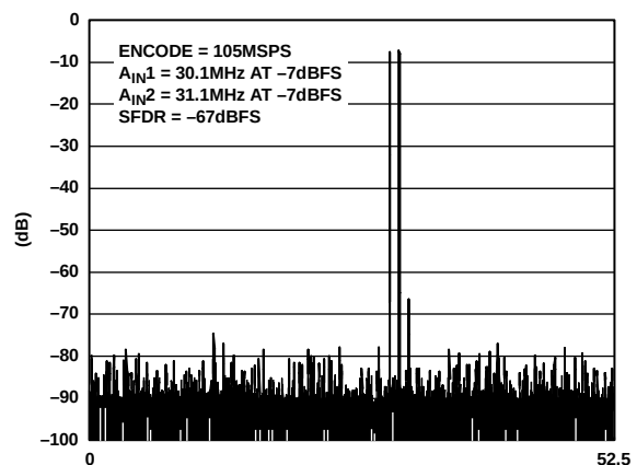
Figure 24. Two-Tone Intermodulation Distortion (30.1 MHz and 31.1 MHz; 1 V p-p, \text{FS} = 105\text{ MSPS} )
