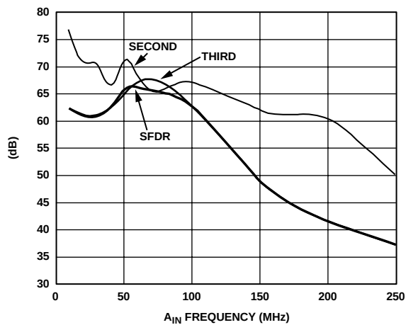
Figure 21. Harmonic Distortion (Second and Third) and SFDR vs. A_{IN} Frequency (1 V p-p, \text{FS} = 105\text{ MSPS} )
