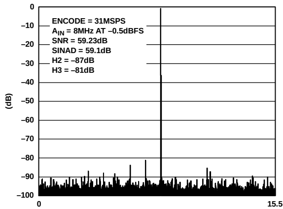
Figure 20. FFT: \text{FS} = 31\text{ MSPS} , A_{IN} = 8\text{ MHz @ } -0.5\text{ dBFS} , Differential, 1 V p-p Input Range
