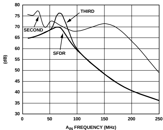
Figure 22. Harmonic Distortion (Second and Third) and SFDR vs. A_{IN} Frequency (1 V p-p, \text{FS} = 80\text{ MSPS} )
