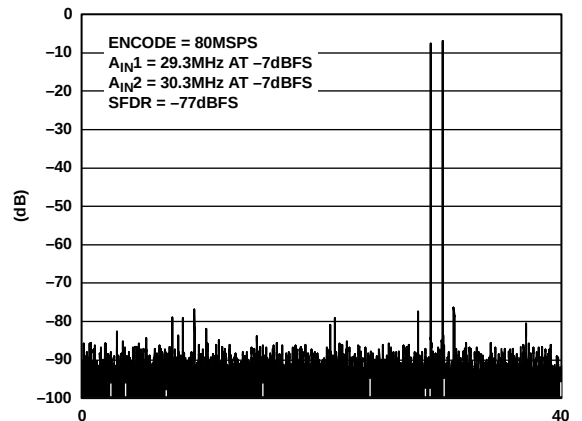
Figure 25. Two-Tone Intermodulation Distortion (29.3 MHz and 30.3 MHz; 1 V p-p, \text{FS} = 80\text{ MSPS} )
