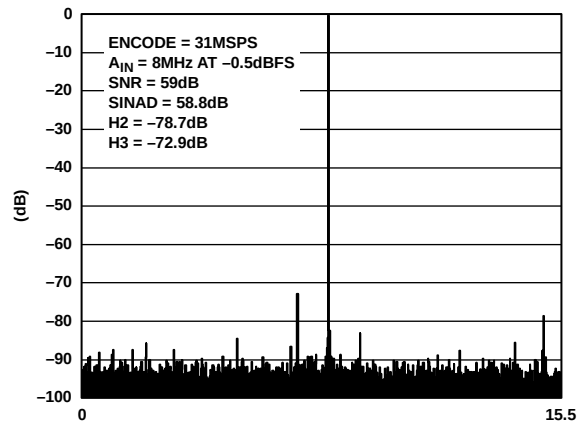
Figure 23. FFT: \text{FS} = 31\text{ MSPS} , A_{IN} = 8\text{ MHz @ } -0.5\text{ dBFS} , Differential, with AD8138 Driving ADC Inputs, 1 V p-p Input Range
