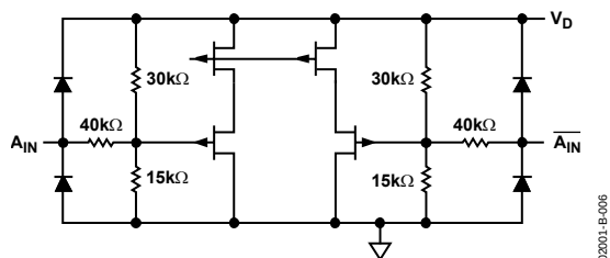
Figure 6. Analog Input Stage
