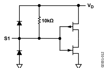
Figure 12. S1 Input
