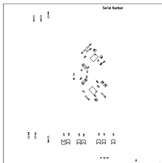
Figure 52. Bottom Silkscreen
