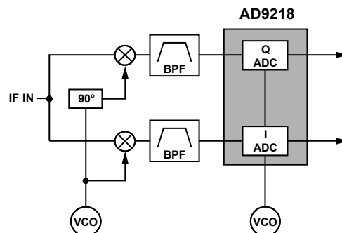
Figure 44. Typical I/Q Demodulation Scheme
