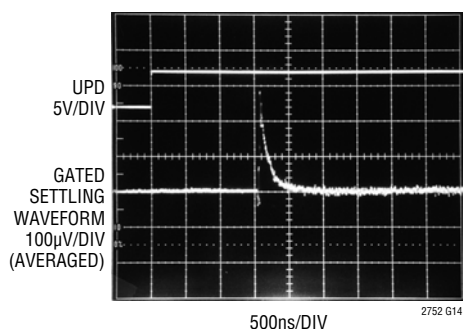
Settling Full-Scale Step
