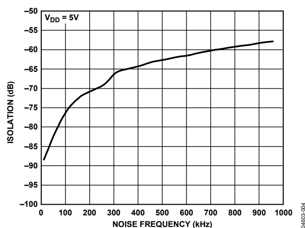
Figure 5. Channel-to-Channel Isolation
