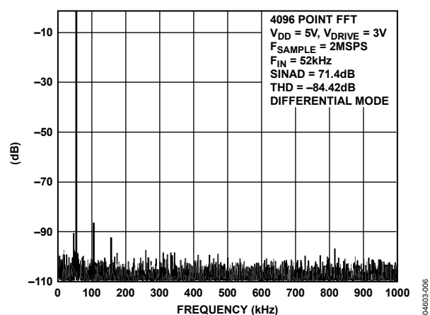
Figure 7. FFT
