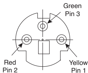
161-2103 3 Pin
