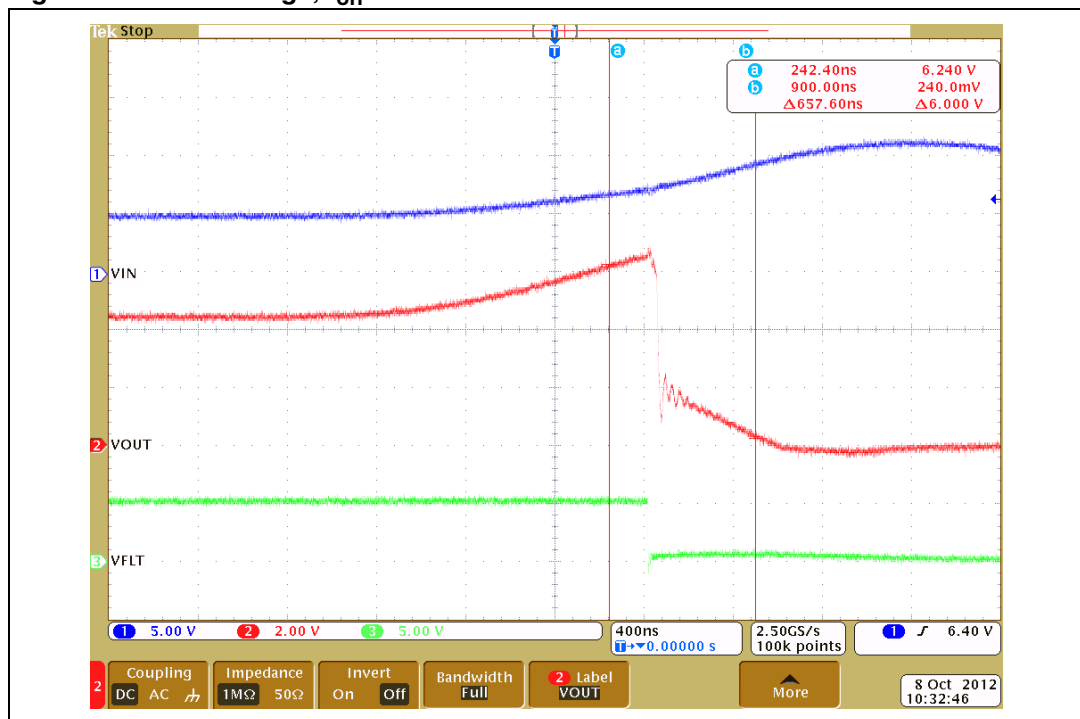
Figure 12. Overvoltage, t_{off}
