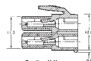
Section X-X
