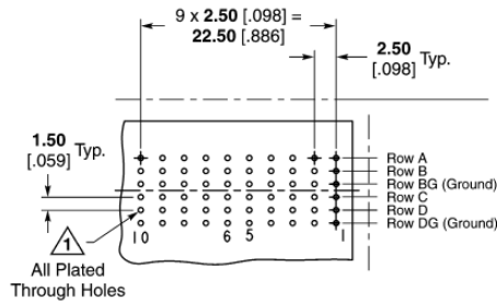
Recommended PC Board Layout Backplane
