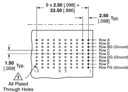
Recommended PC Board Layout Backplane, Component Side Shown
