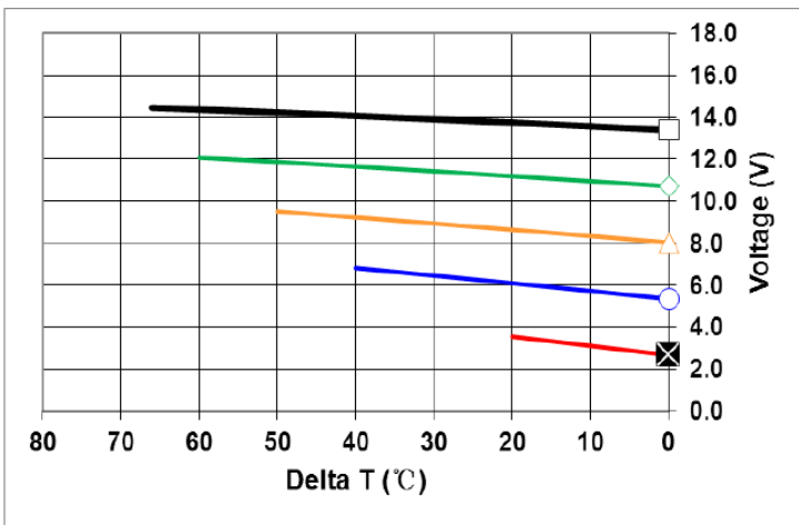
Performance Curves Th=25 °C
