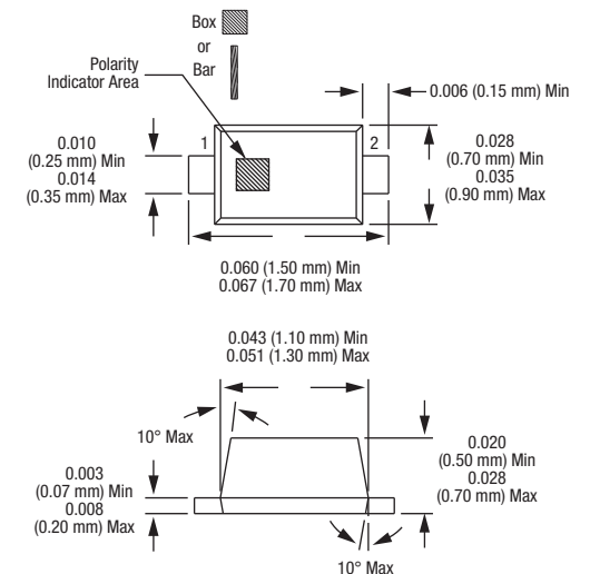
Figure 7. SC-79 Package Dimension Drawing
