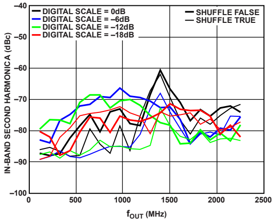
Figure 71. SFDR for In-Band Second Harmonic vs. f_{OUT} over Digital Scale
