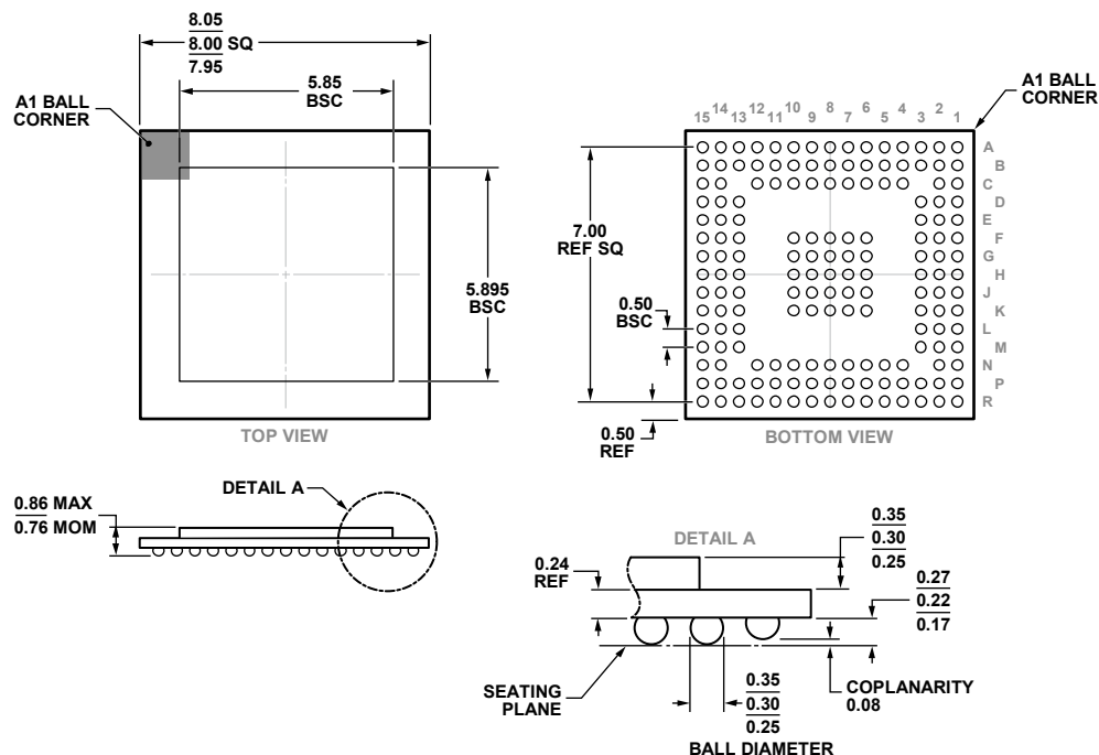
Figure 195. 165-Ball Chip Scale Package Ball Grid Array [CSP_BGA] (BC-165-1)
